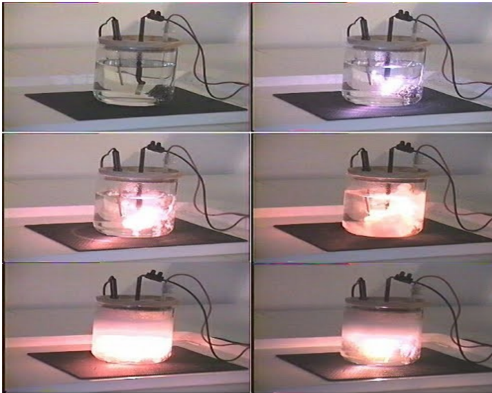
Cold Fusion Reactor v1.0 build and tested by Jean-Louis Naudin Based on Mizuno-Ohmori experiment - May 7th, 2003 Email: Jnaudin509@aol.com - http://www.jlnlabs.org
